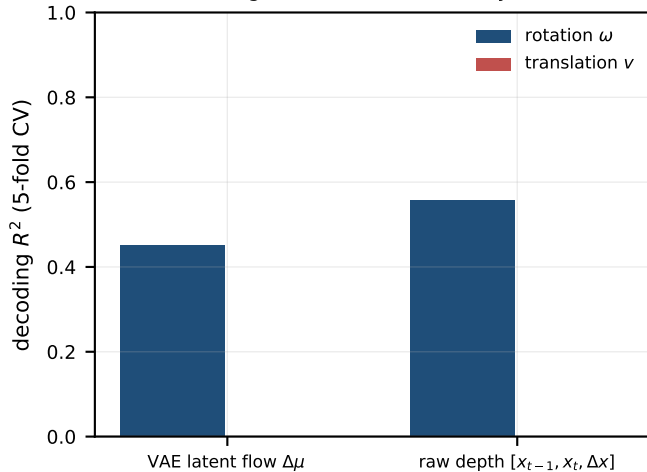
ego-motion recoverability
