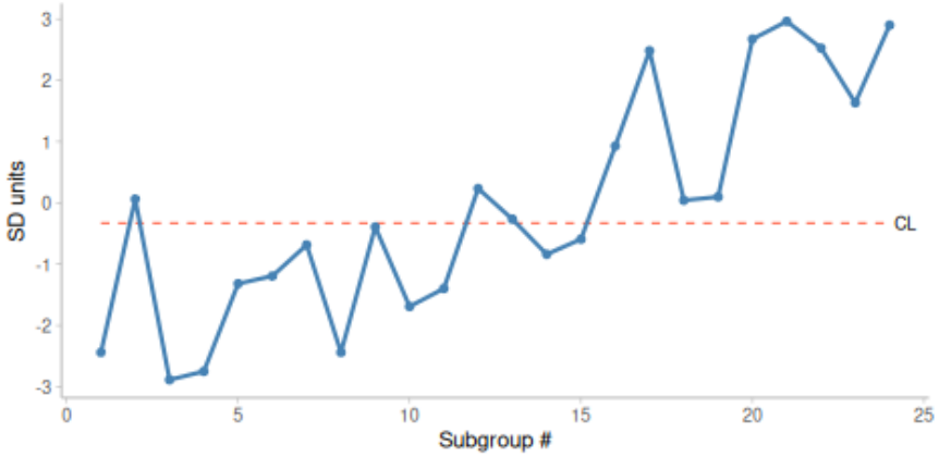
Figure 3.6: Run chart with a trend
