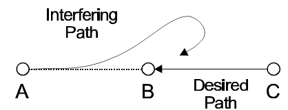
Spatially Uncorrelated
