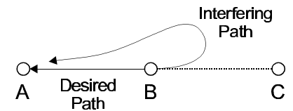
Spatially Correlated
