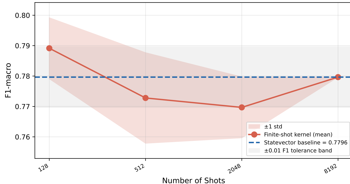
(a) F1-macro convergence to statevector baseline
