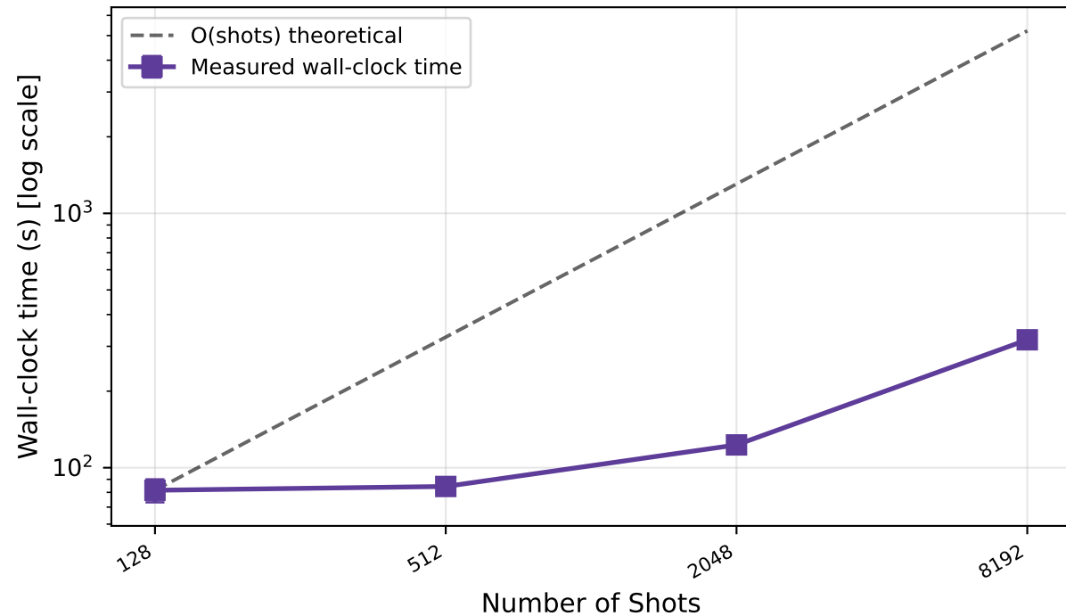
(a) Kernel Matrix Computation Time vs Shots
