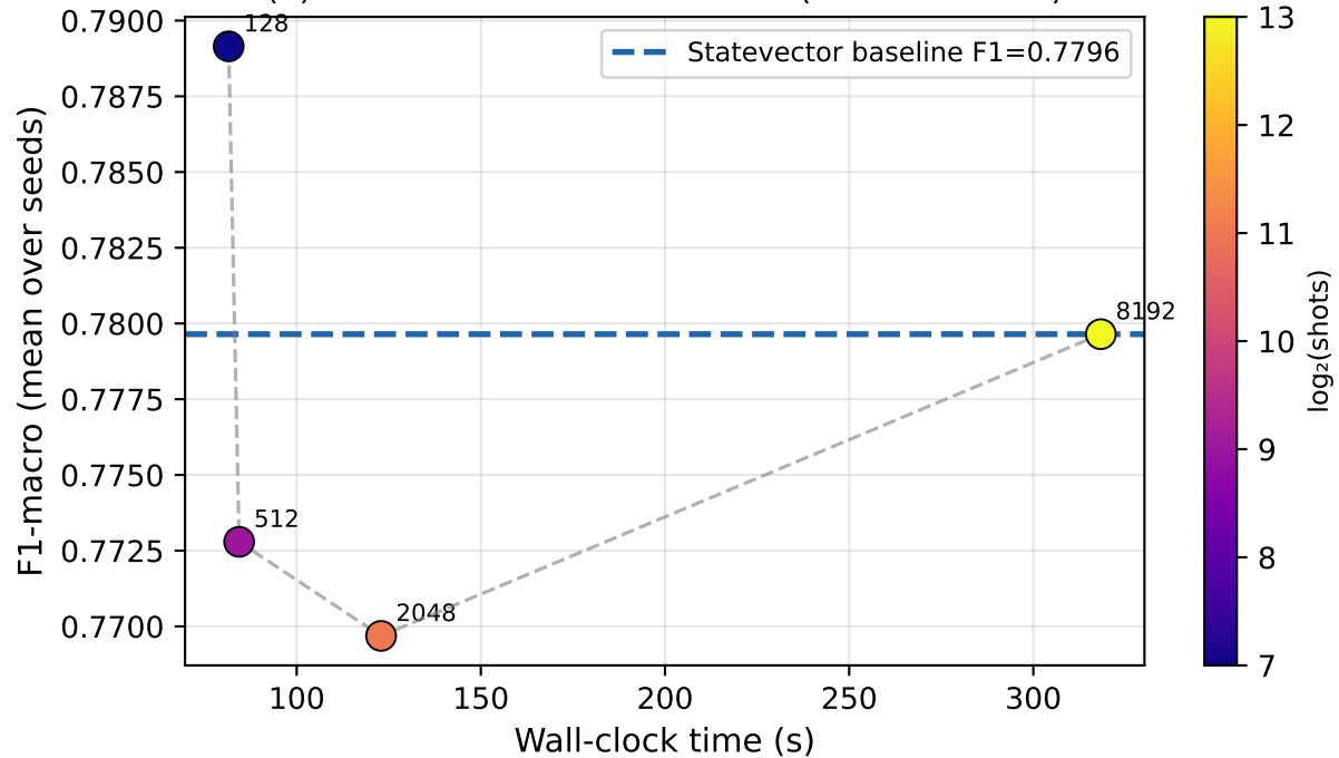
(b) F1-macro vs Wall-clock Time (Pareto Frontier)
