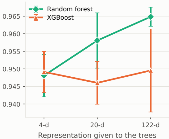
(a) Ranking: AUC-PR higher is better
