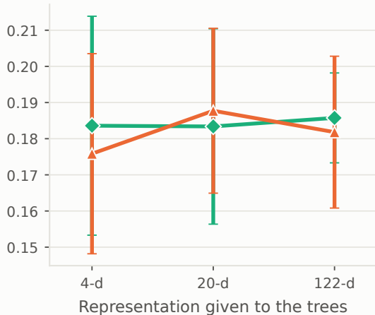
(b) Calibration: ECE lower is better
