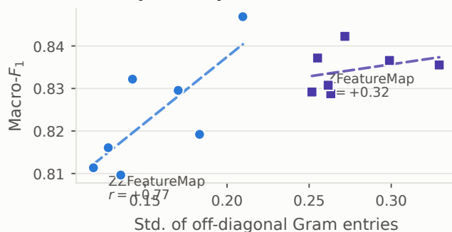
(c) Dispersion predicts F_1
