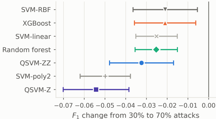
(b) Degradation under the shift
