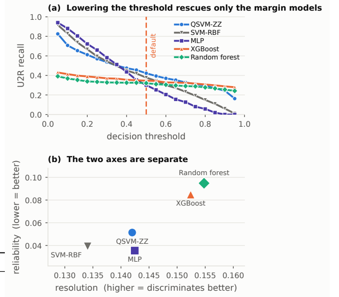
Fig. 6. (a) U2R recall against the decision threshold. The margin-based models recover the rare class as the threshold falls; the tree ensembles do not. (b) The Murphy decomposition separates the two axes: the tree ensembles sit top-right, discriminating best and calibrating worst.
