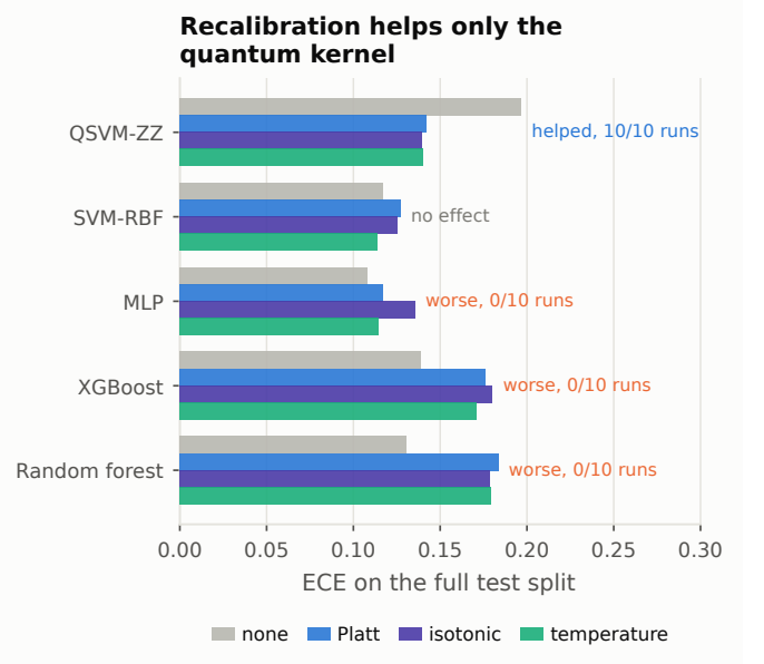
Fig. 5. Post-hoc recalibration helps the quantum kernel in all 10 runs, degrades the MLP and both tree ensembles in all of them, and leaves the RBF kernel unchanged. The labels are the Holm-corrected paired verdicts of Table VI rather than a comparison of means: the RBF kernel's mean does improve under temperature scaling, but it wins in only 5/10 runs.
