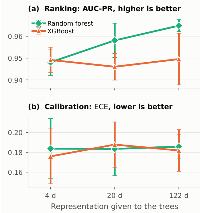
Fig. 4. Giving the tree ensembles a richer representation, with every hyper-parameter held fixed. Ranking improves; calibration gets worse.
