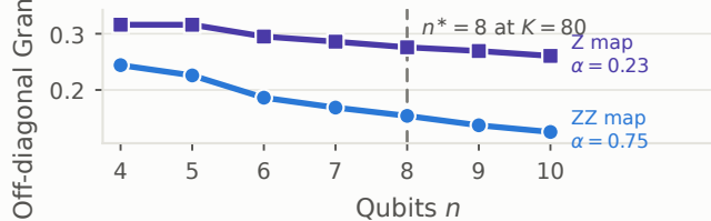
(b) The kernel concentrates as n grows
