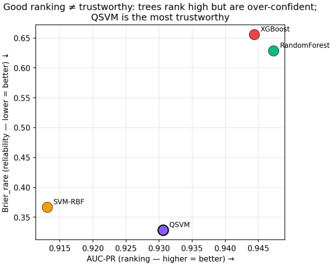
Fig. 5. Ranking quality (AUC-PR) versus trustworthiness (Brier rare ). Tree ensembles rank well but are over-confident; QSVM-ZZ is the most trustworthy.
