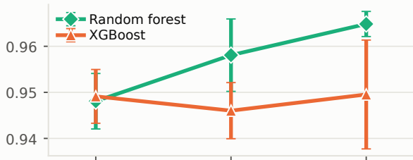
(a) Ranking: AUC-PR, higher is better
