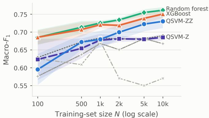
(a) UNSW-NB15 learning curve, natural prior
