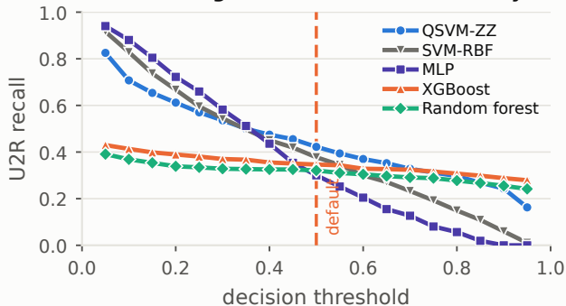
(a) Lowering the threshold rescues only the margin models
