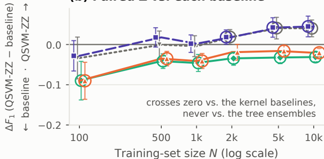
(b) Paired \Delta vs. each baseline
