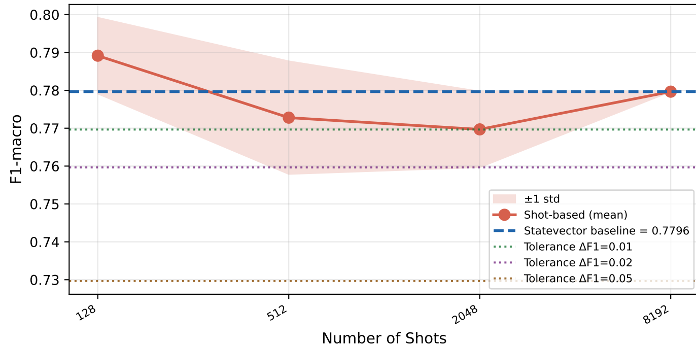
(a) Convergence of F1-macro to Statevector Baseline
