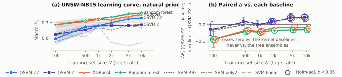
Fig. 7. What transfers to UNSW-NB15, and what does not. (a) Mean macro- F_1 over ten runs on the official test set; (b) paired differences, circled where the Holm-adjusted p < 0.05 . The selection rule and the entanglement ablation transfer; the sample-complexity crossover does not. Against both tree ensembles the difference keeps its sign at every N , the opposite of NSL-KDD.
