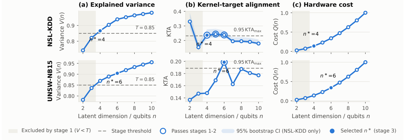
Fig. 1. The three-stage dimension-selection rule, applied unchanged to two datasets. Rows: NSL-KDD (top), UNSW-NB15 (bottom). Columns: (a) cumulative explained variance V(n) , (b) kernel-target alignment, (c) CNOT-weighted cost Q(n) . Stage 1 discards V(n) < 0.85 (shaded), stage 2 keeps KTA \geq 0.95 KTA_{\max} (open circles), stage 3 takes the cheapest survivor (filled). The same rule returns n^* = 4 and n^* = 6 .
