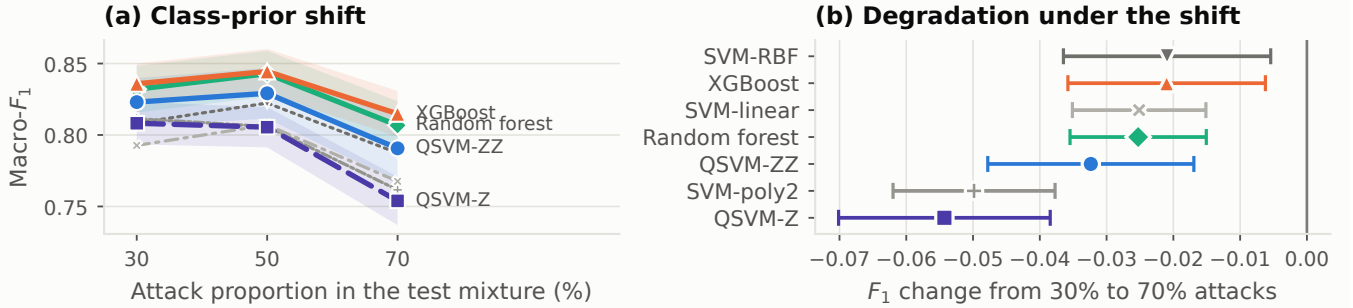
Fig. 5. Under class-prior shift the quantum kernel degrades more than the tree ensembles, not less. (a) Macro- F_1 as the attack proportion moves from 30% to 70%, over ten runs with 95% bands (models trained on the N = 1000 rare-enriched subsets; test mixtures of 1000 records). (b) The paired change across that shift, sorted. QSVM-zz loses 0.032 against 0.021 for XGBoost and 0.025 for the random forest. The submitted version named this regime as its strongest evidence.
