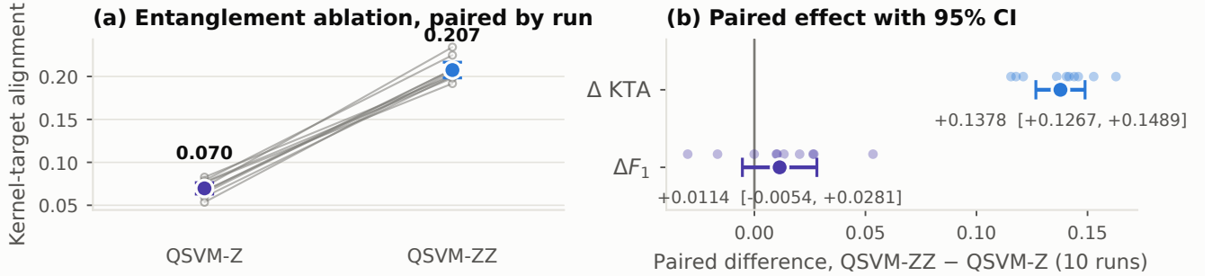
Fig. 3. Entanglement moves the kernel geometry far more than it moves the score. (a) Kernel-target alignment for the two feature maps, paired within each of ten runs ( N = 1000 , rare-enriched pool, 300-record test split). (b) The paired differences. Removing the entangling layer costs 0.1378 alignment [0.1267, 0.1489], an interval far from zero, but only 0.0114 macro- F_1 [-0.0054, 0.0281], an interval that contains it.
