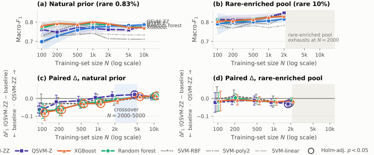
Fig. 6. Rare-attack enrichment, not sample size alone, decides whether the quantum kernel leads on NSL-KDD. (a, b) Mean macro- F_1 over ten runs on the full KDDTest+ set with 95% bands; (c, d) paired differences against each baseline, circled where the Holm-adjusted p < 0.05 . Under the natural prior the ordering reverses between N = 2000 and N = 5000 (band in c). Twelvefold rare enrichment removes the reversal (d).
