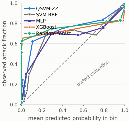
(a) Reliability diagram, KDDTest+
