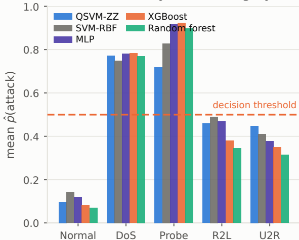
(b) Confidence by attack category
