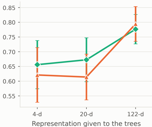
(b) Reliability: ECE_{rare} lower is better
