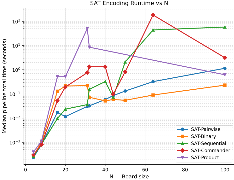
Figure 3: SAT Runtime vs N
