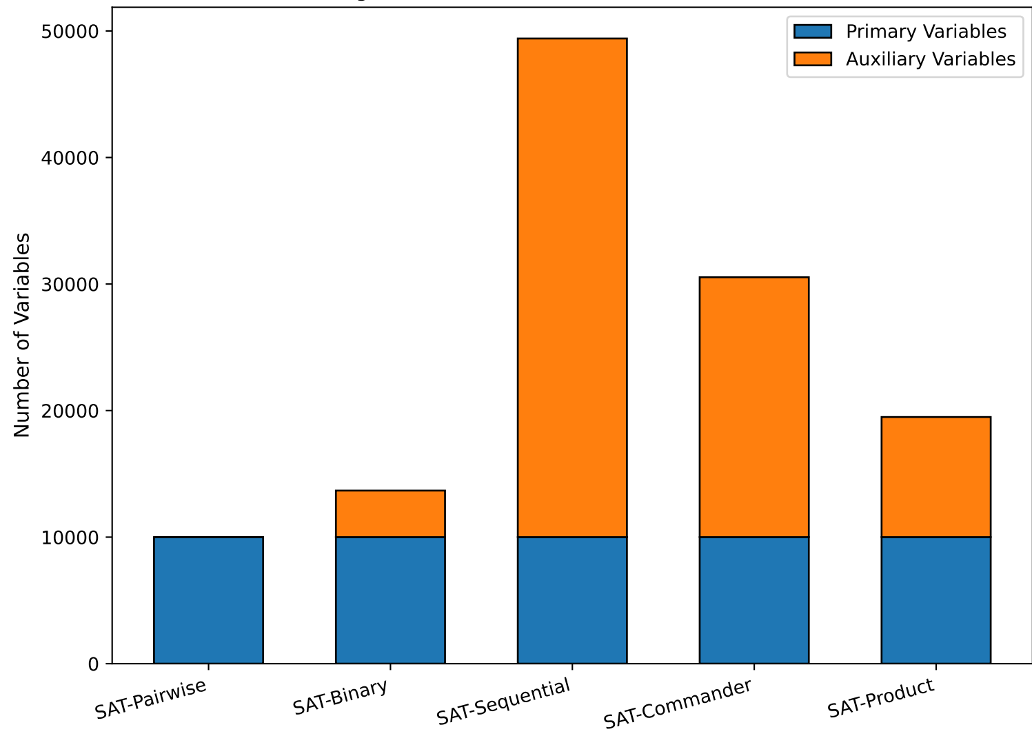
Figure 5: SAT Variable Overhead at N=100
