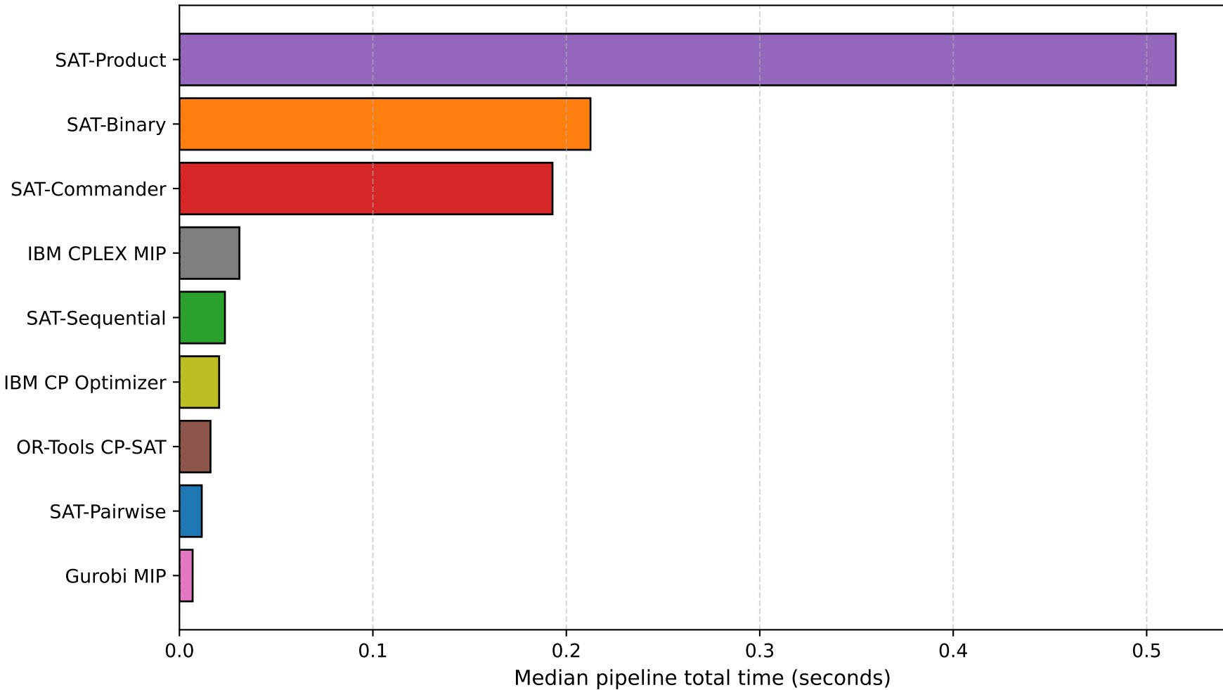
Figure 3: All-Nine-Method Comparison at N=20
