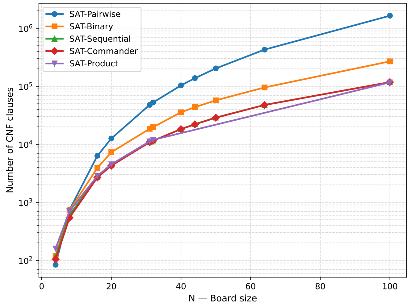
CNF Clause Growth vs N
