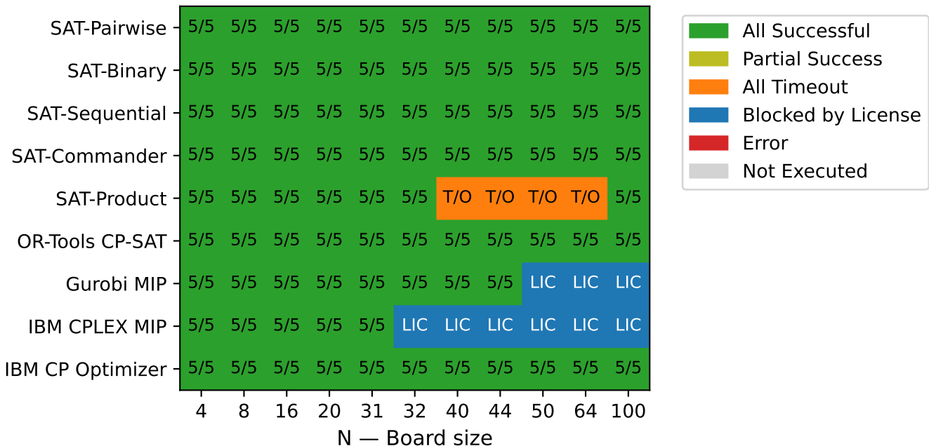
Completion / Timeout Matrix
