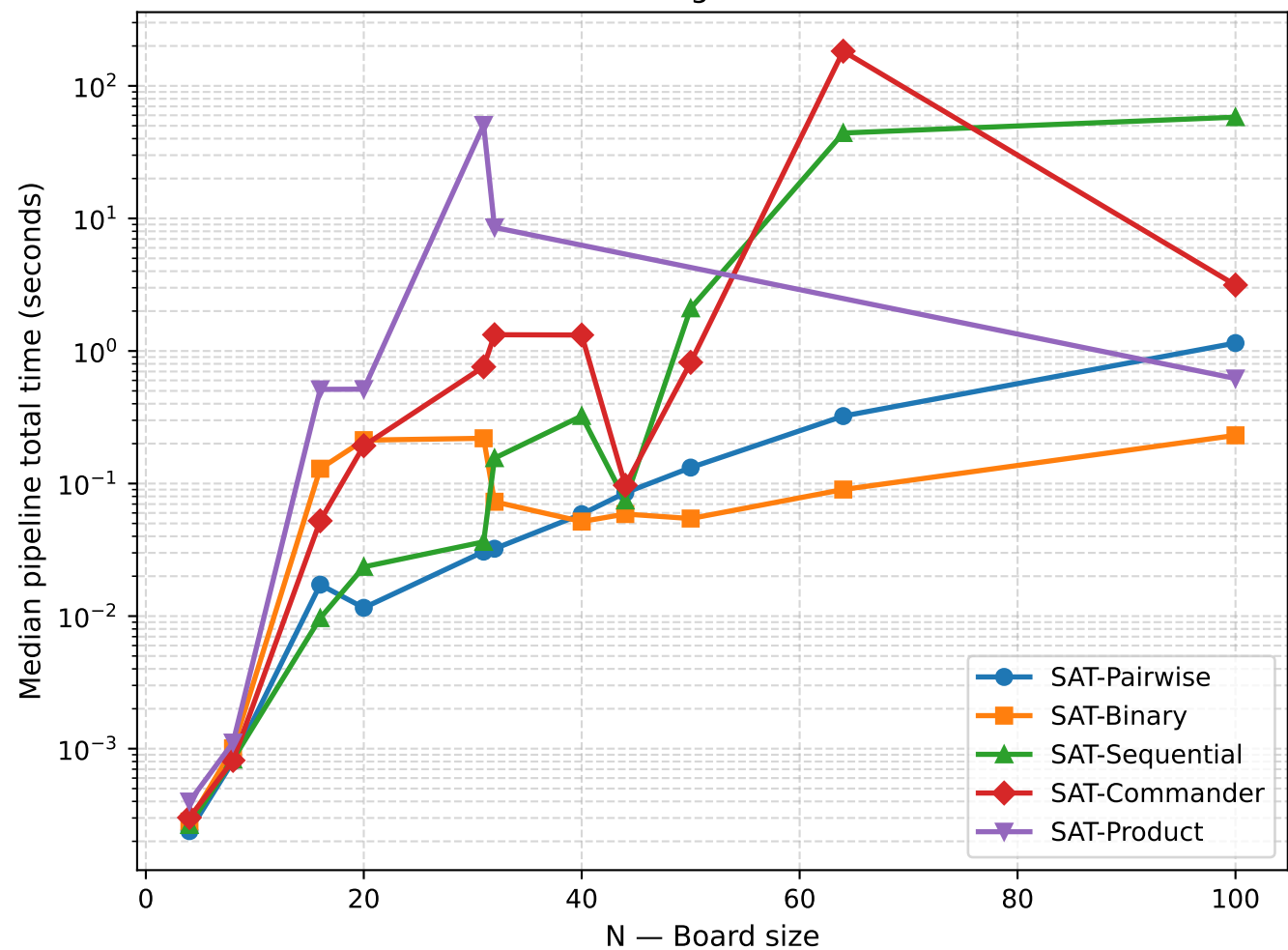
SAT Encoding Runtime vs N
