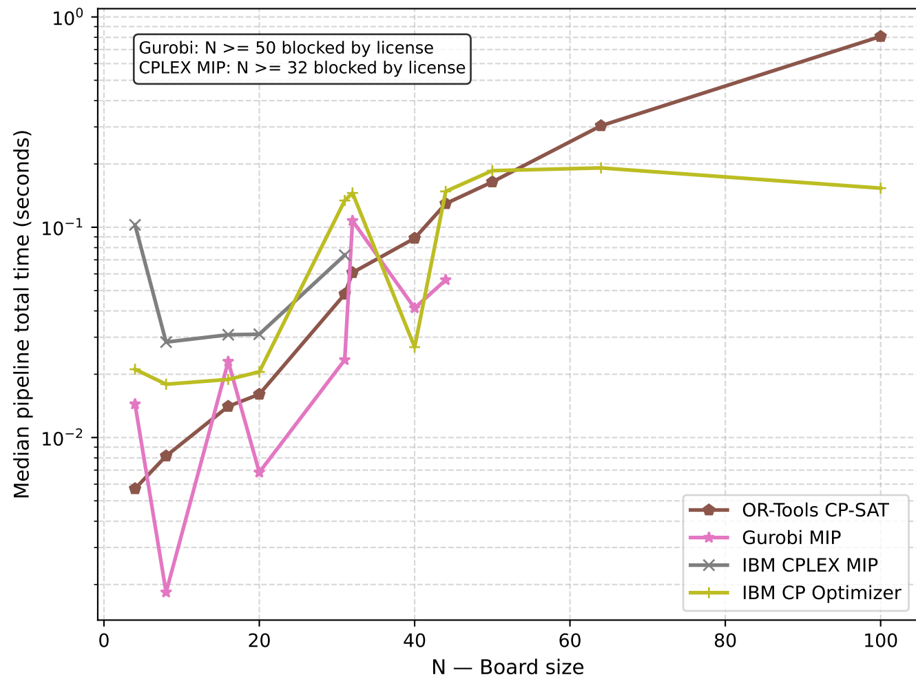
Exact Solver Runtime vs N
