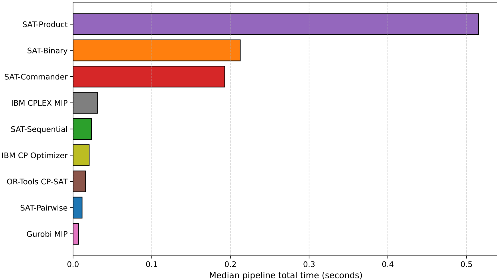
All-Nine-Method Comparison at N=20
