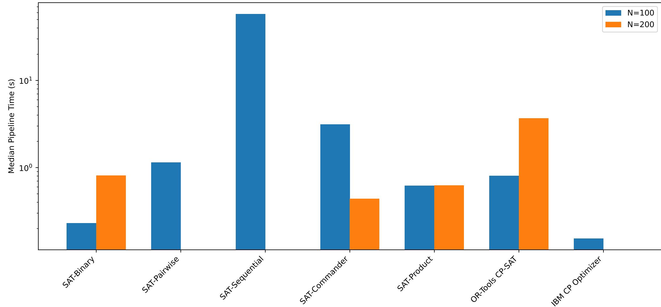
Runtime Comparison at N=100 and N=200
