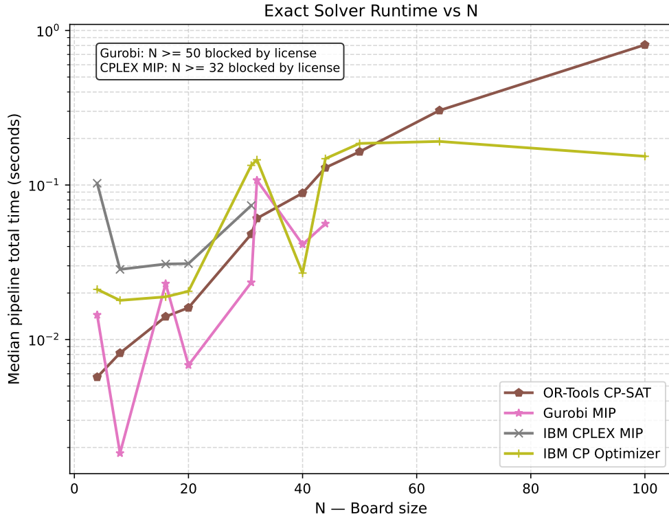
Figure 5: Exact Solver Runtime vs N
