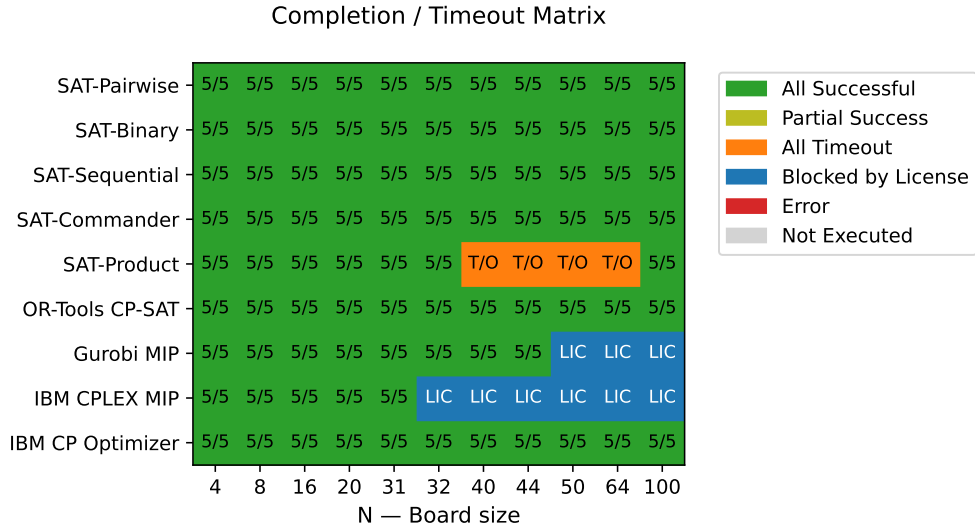
Figure 4: Completion Matrix
