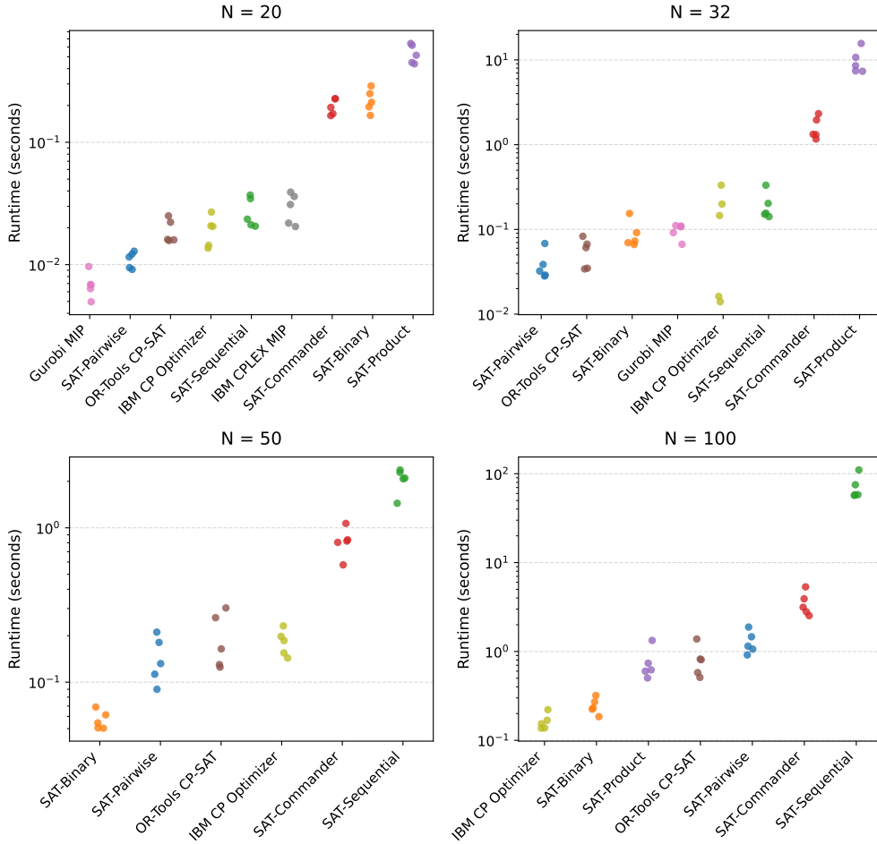
Figure 6: Runtime Variability
