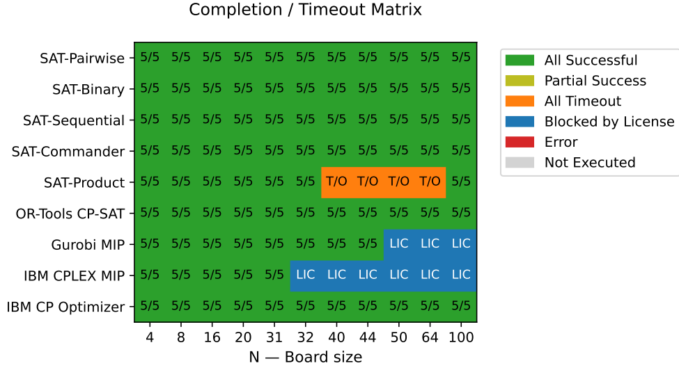
Figure 4: Completion Matrix
