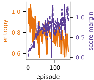
(c) Policy sharpens
