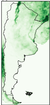
(c) MODIS v6.1 2023
