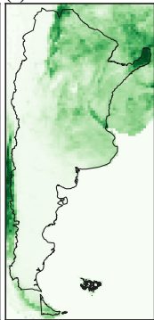
(b) MODIS v6.1 2003
