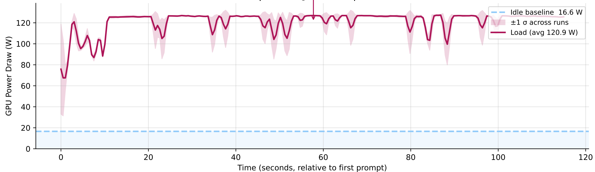
GPU Power Timeline — gemma3:4b (3 runs averaged) Idle: 16.6 W | Load avg: 120.9 W | \Delta = +104.3 W
