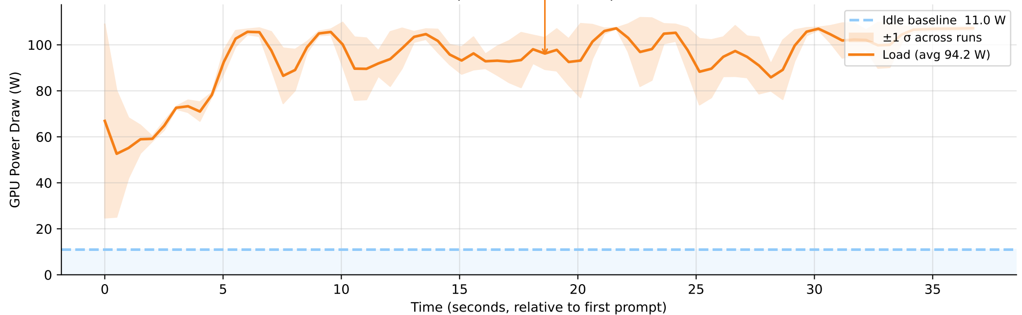
GPU Power Timeline — llama3.2:1b (3 runs averaged) Idle: 11.0 W | Load avg: 94.2 W | \Delta = +83.2 W
