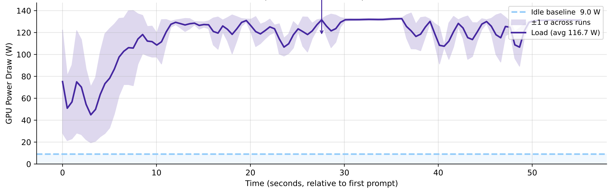
GPU Power Timeline — llama3.2:3b (3 runs averaged) Idle: 9.0 W | Load avg: 116.7 W | \Delta = +107.7 W
