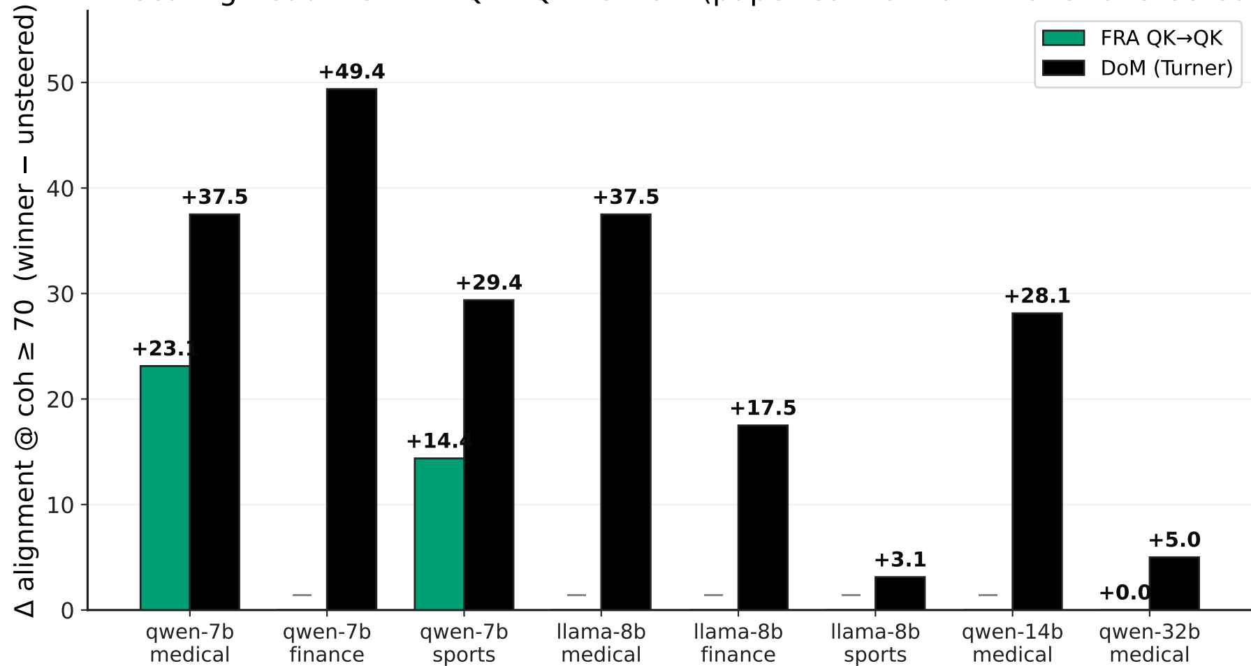
EM-scaling headline: FRA QK→QK vs DoM (paper convention: \Delta over unsteered)
