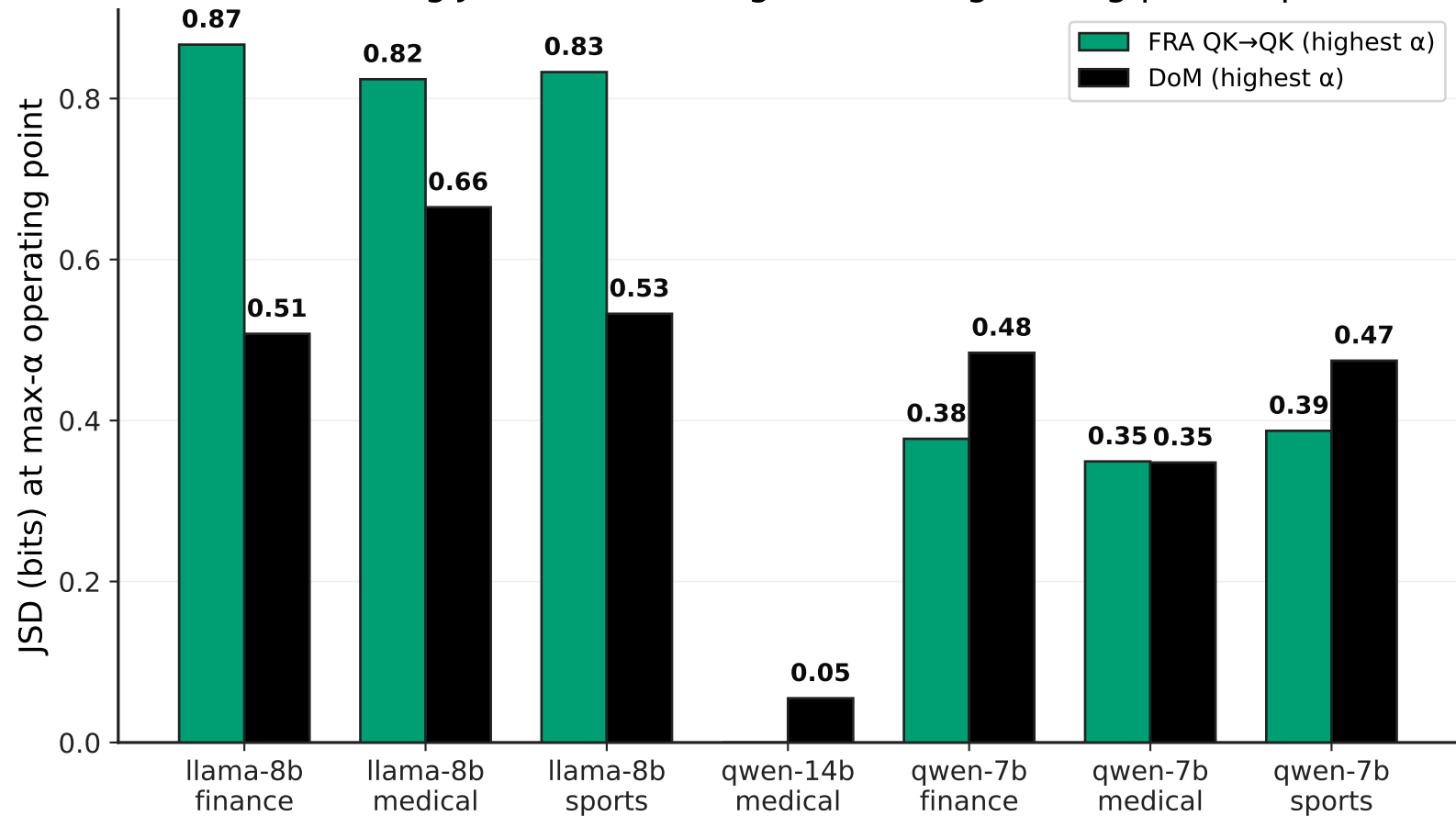
EM-scaling JSD at the strongest steering setting per recipe
