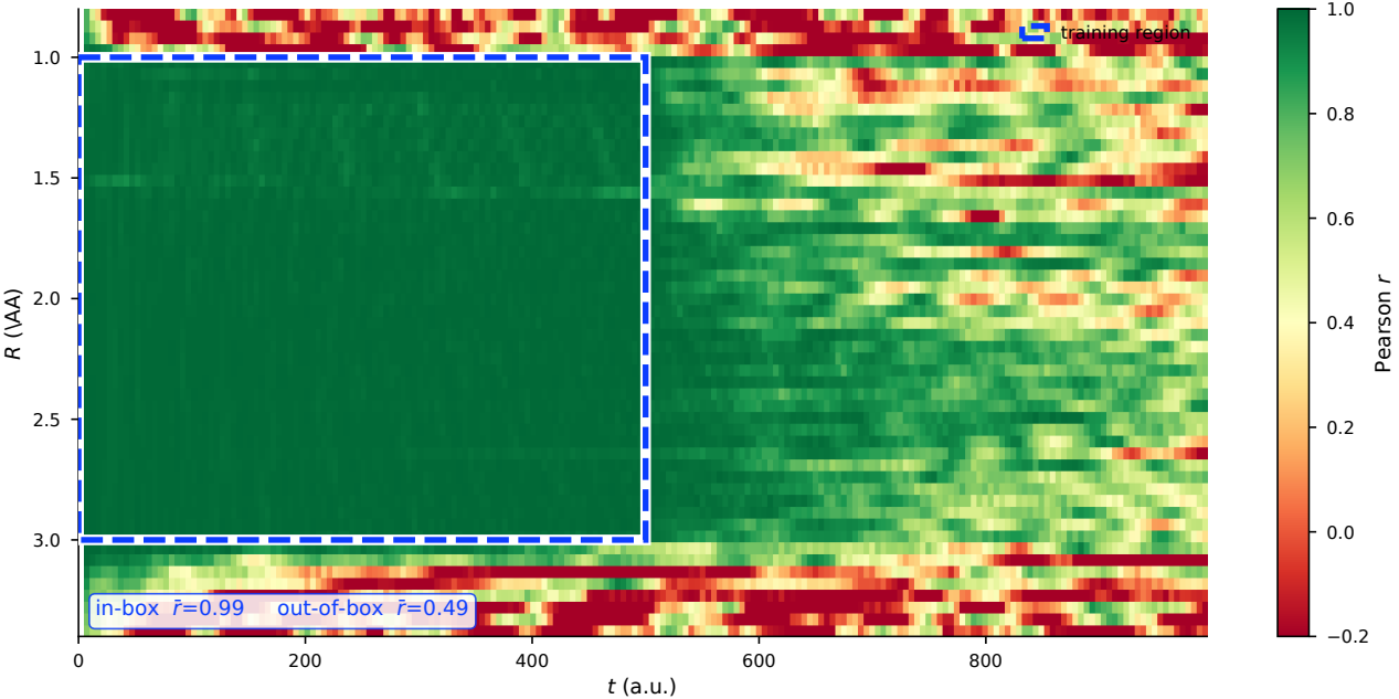
Windowed Pearson r(R, t) --- model vs. \ exact observables
