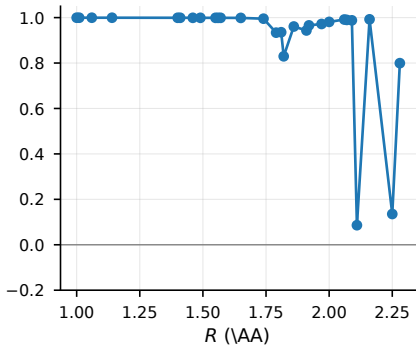
Observable correlation vs R
