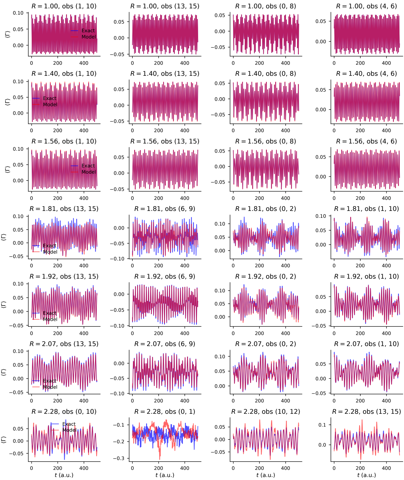
Observable time series: Model (red) vs Exact (blue)
