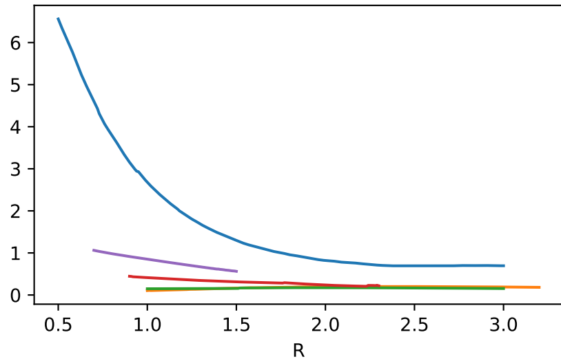
temporal-bandwidth S_t(R)
