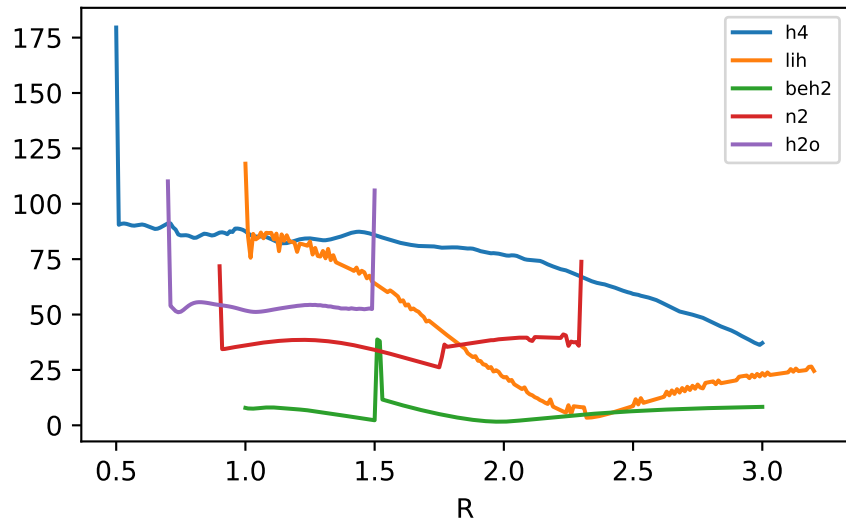
geometry-smoothness S_R(R)
