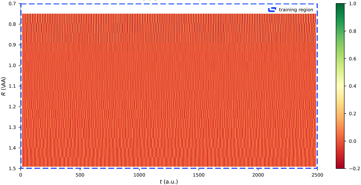
Windowed Pearson r(R, t) --- model vs. \ exact observables
