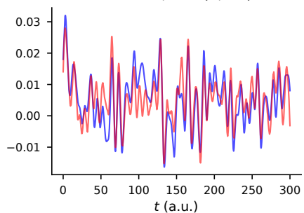
R = 2.93 , obs (8, 10)
