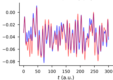
R = 2.93 , obs (0, 7)
