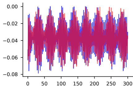
R = 1.95 , obs (11, 15)
