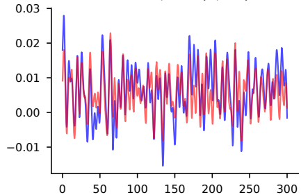
R = 2.93 , obs (8, 10)
