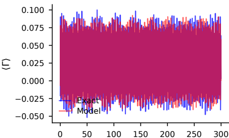
R = 1.95 , obs (6, 9)
