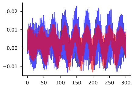
R = 1.95 , obs (8, 10)
