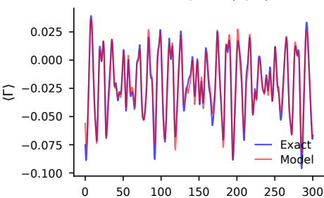
R = 2.93 , obs (6, 7)
