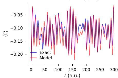
R = 2.93 , obs (6, 7)
