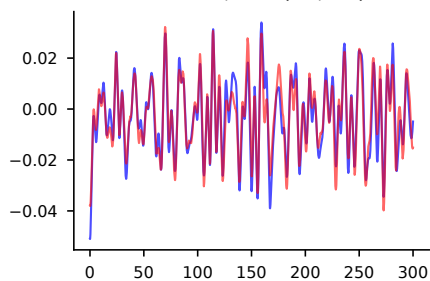
R = 2.93 , obs (0, 7)
