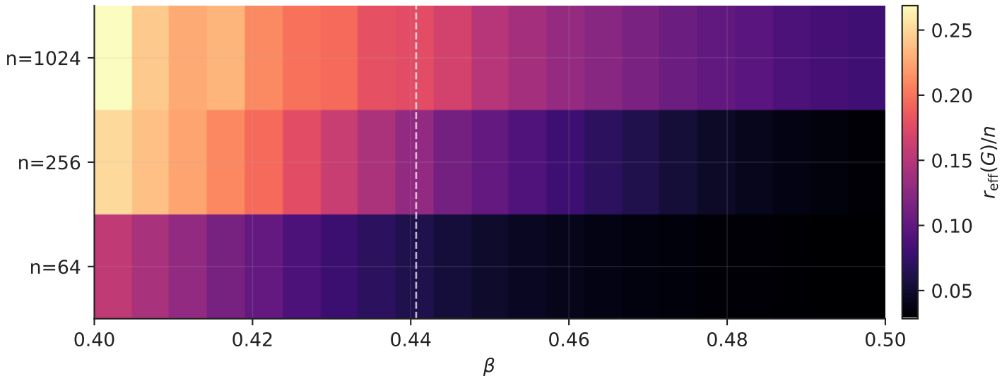
effective rank phase map (tier6)
