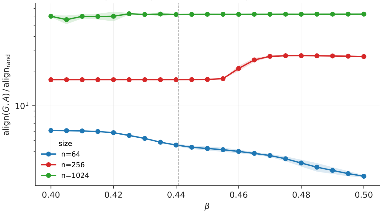
phase diagram of *relative* alignment (tier6)
