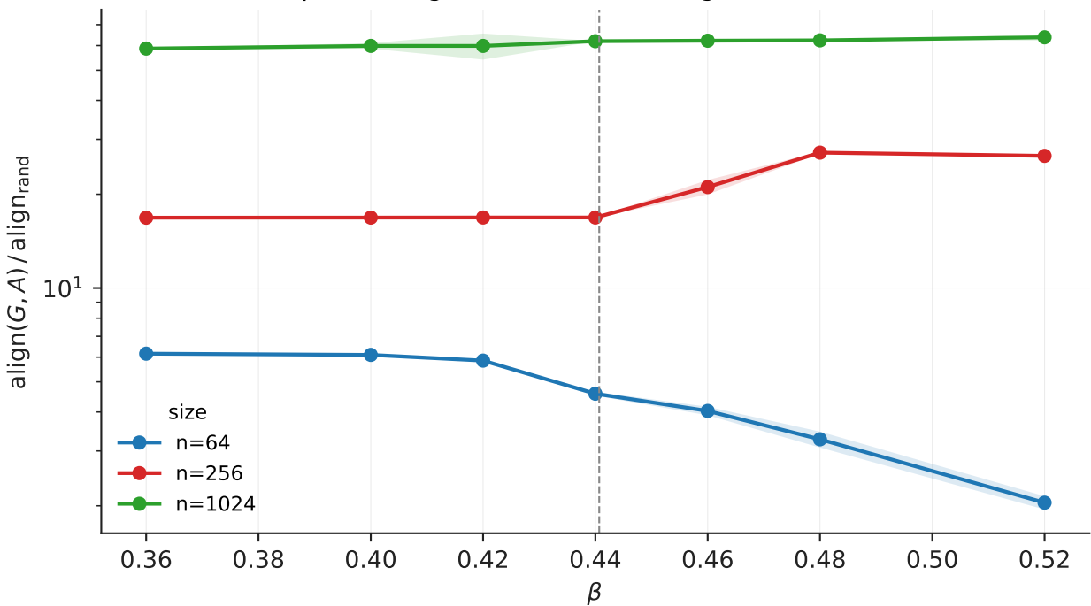
phase diagram of *relative* alignment (tier4)
