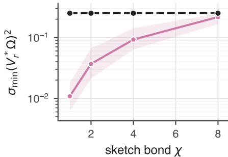
injection vs sketch bond ( L_x=8 )
