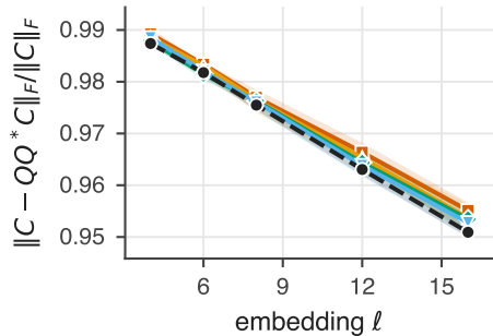
column error vs \ell ( L_x=8 )
