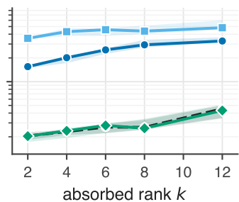
Wall-clock (secondary)
