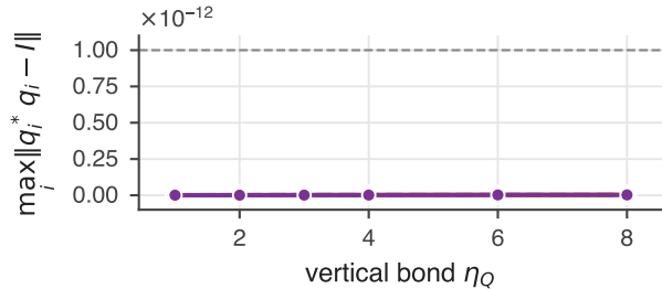
Arrow isometry defect
