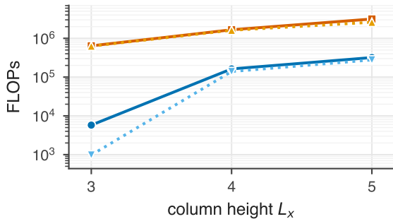
Column-factorization FLOPs
